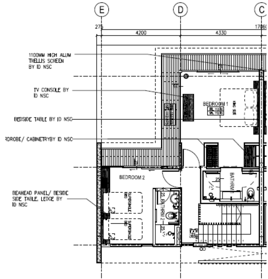
VILLA A/B 2ND STOREY PLAN
